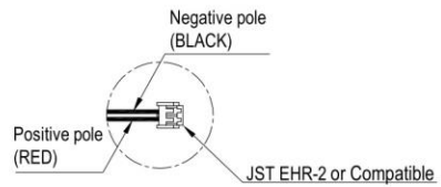
Connector View
